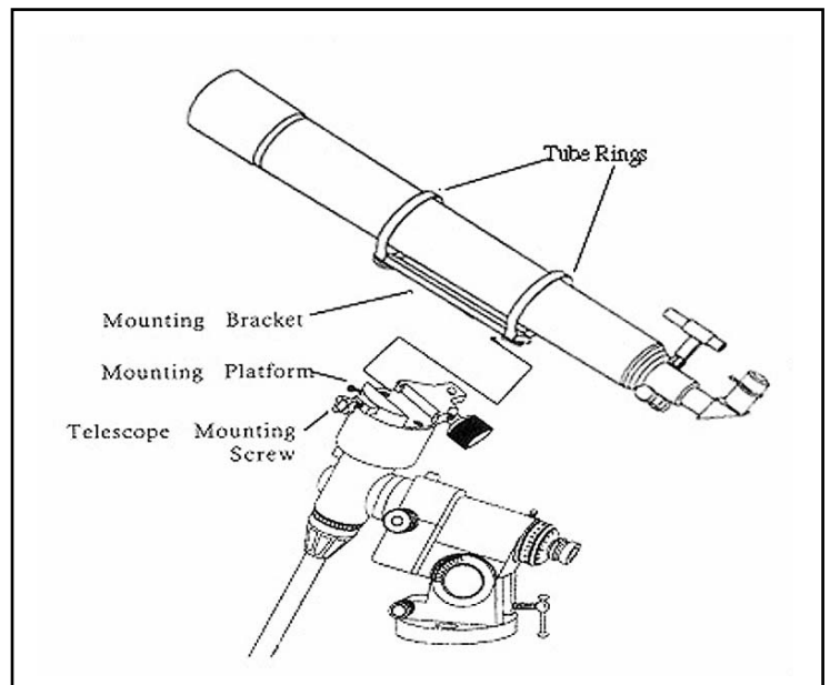
Figure 2-9 Refractor Optical Tube is shown. The Newtonian and Schmidt-Cassegrain attach similarly.
